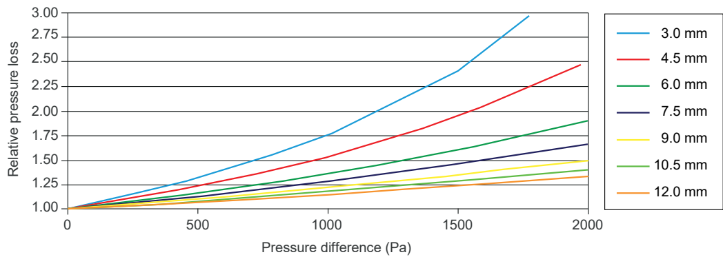
Figure 1. Effect of pressure difference on pressure loss, Model H.
