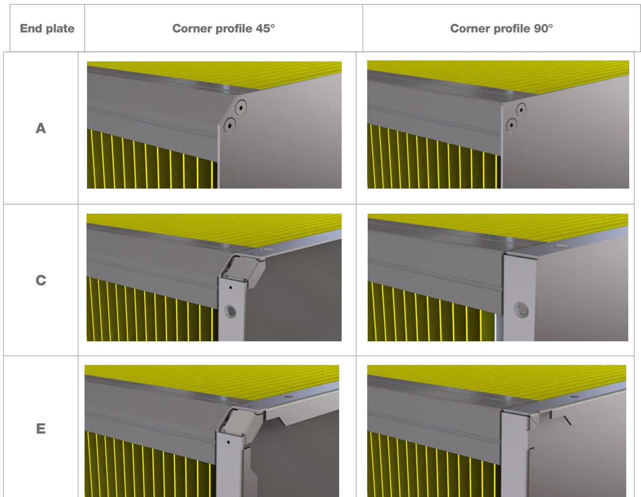
Image 10. End plates and corner profiles
