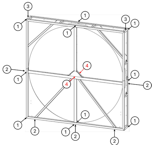
Image 29. Forces - Vertical plane of intersection
