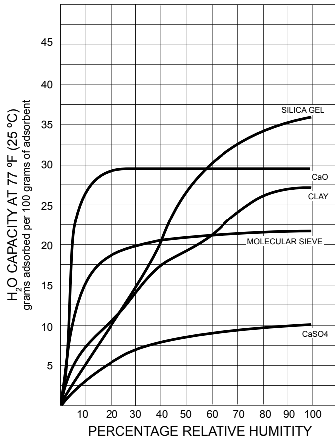
Image 2. Adsorption rate (H2O) of various adsorbents.
