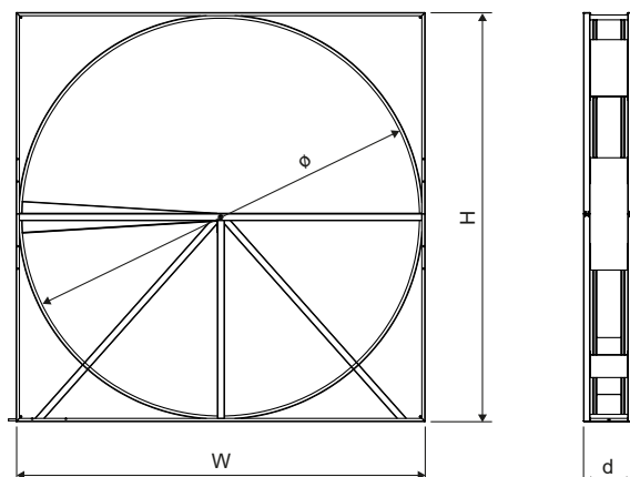
Image 31. Model ES casing dimensions
