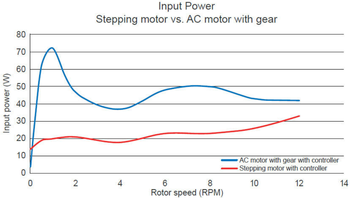
Image 25. Input power vs rotor speed for a gearbox motor and a step motor.
