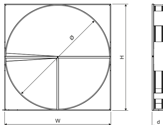
Image 20. Model E casing types small, medium and large.
