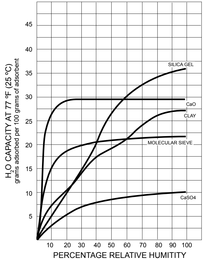
Image 2. Adsorption rate (H2O) of various adsorbents.
