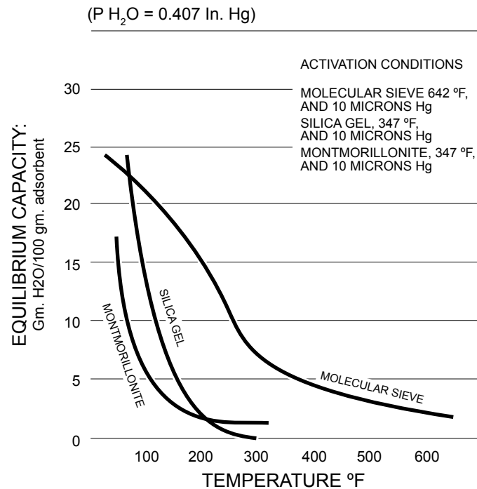
Image 3. Equilibrium capacity (H 2 O) of various adsorbents.
