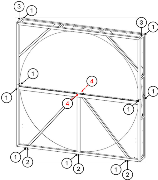
Image 26. Forces - Horizontal plane of intersection
