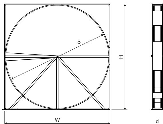
Image 29. Model ES casing dimensions
