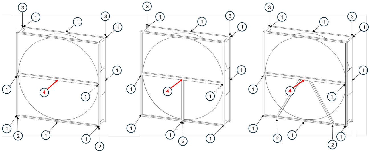
Image 17. Vertical top/ bottom airflow.
