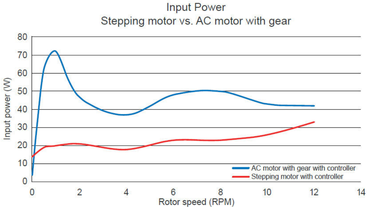
Image 23. Input power vs rotor speed for a gearbox motor and a step motor.
